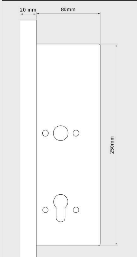
Standard lock-cassette dimensions
