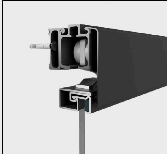
Wall mounted sliding rail
